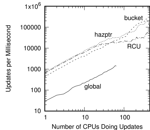
Figure 10.12: Update-Side RCU-Protected Hash-Table Performance For Schrödinger's Zoo
